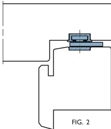
HORIZONTAL PLANE
